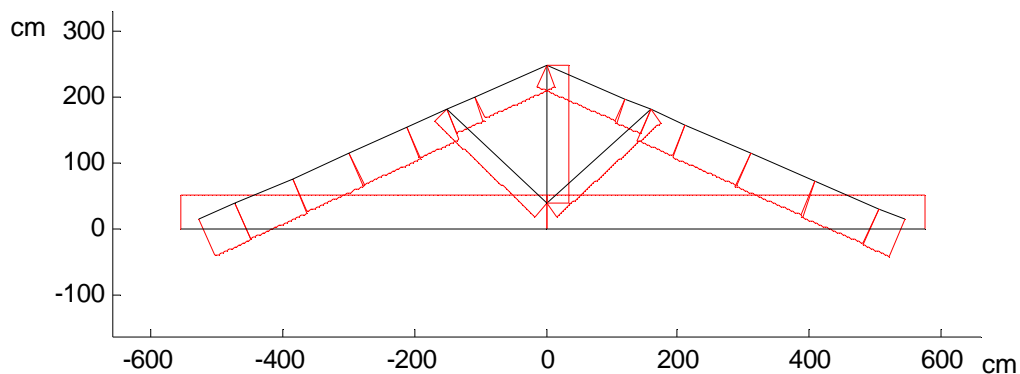
Axial force (Nx)
