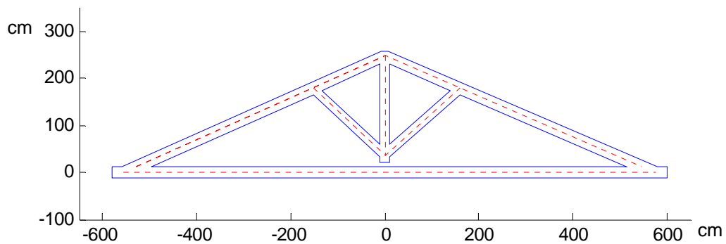
Truss geometry and beam axes
