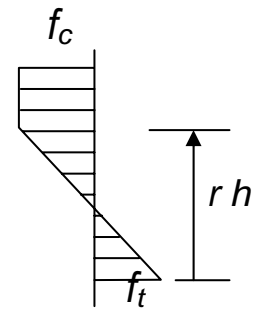
stress distribution at the ultimate limit state of a cross section
