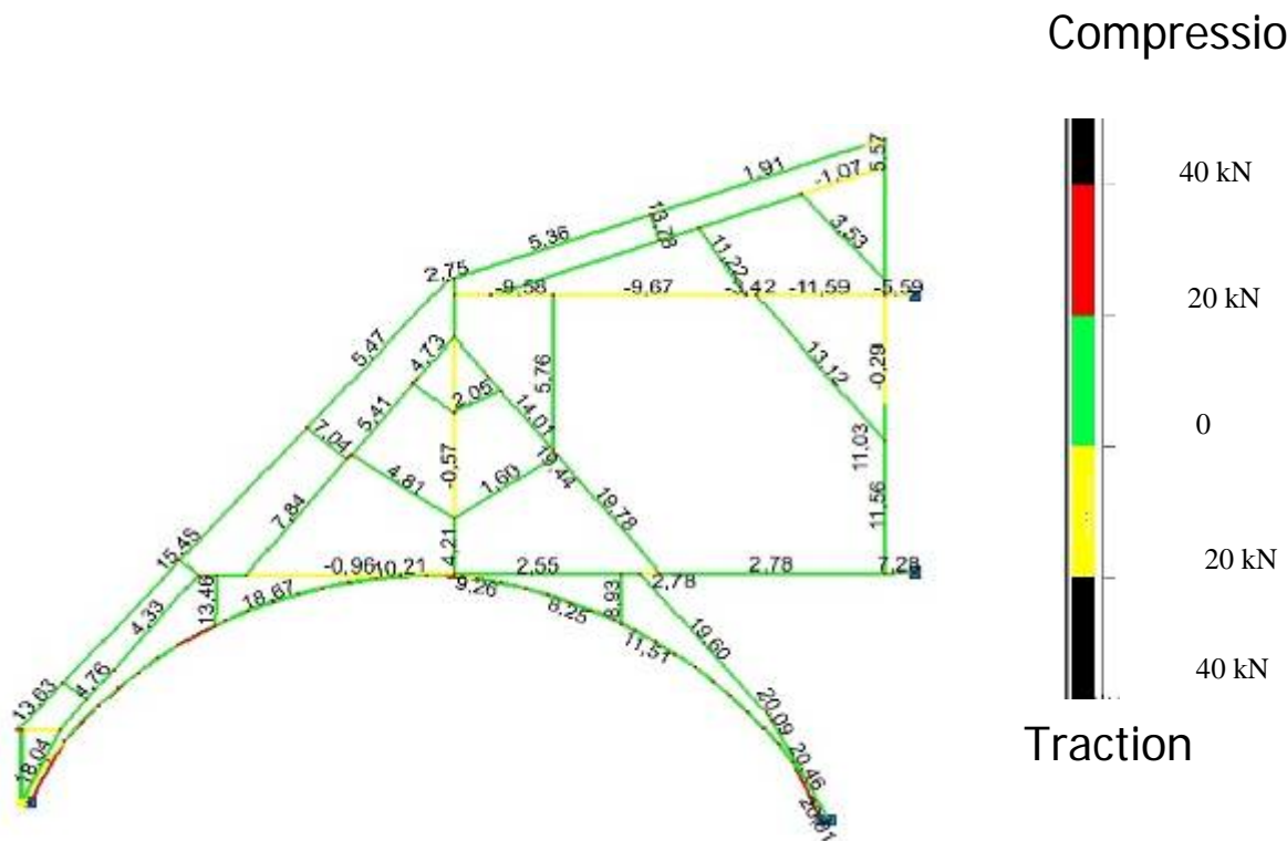
Normal strain in the bars (in kN)
