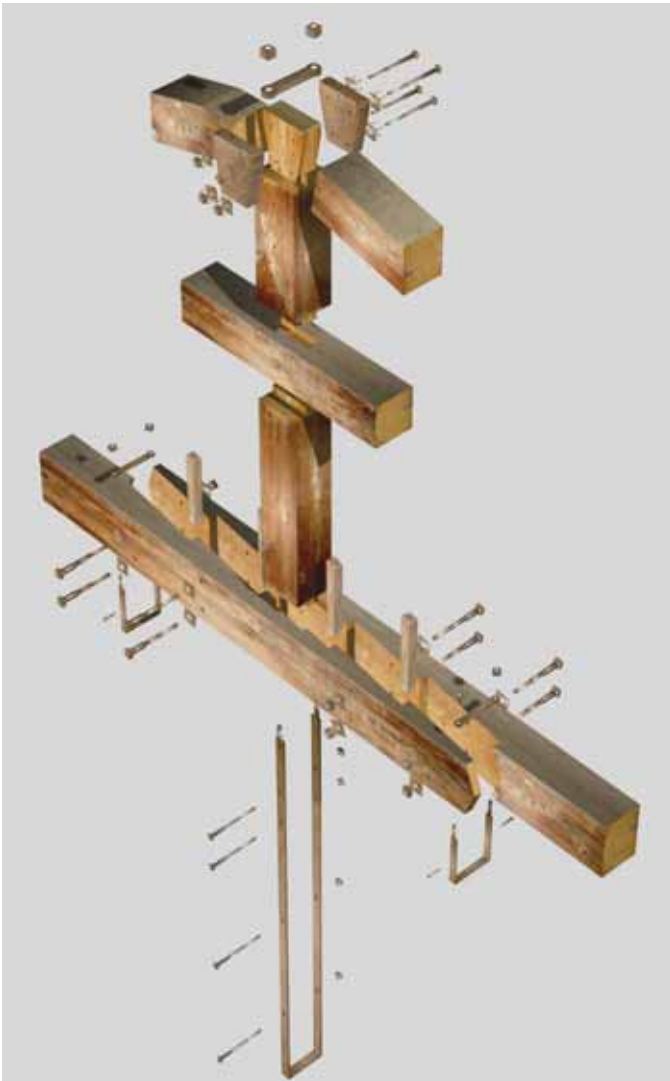
Figure 2: Exploded axonometric view of the node: king post-rafter-chord of the Giraldi's truss
