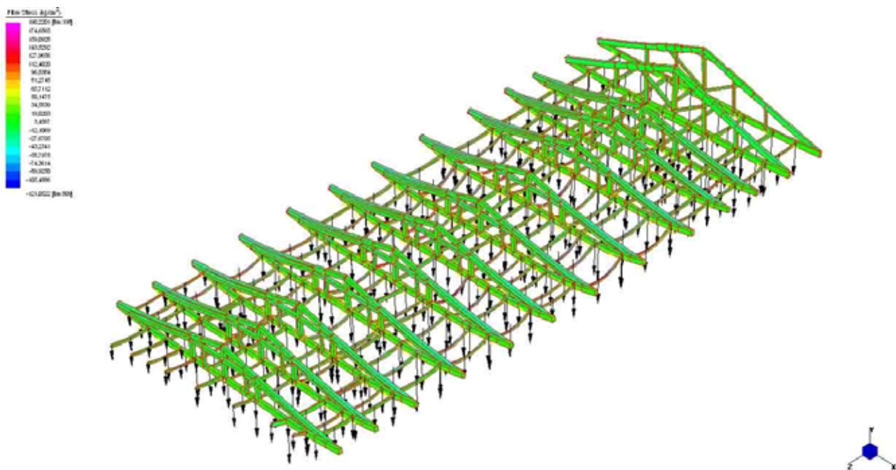
Figure 4: Stresses and displacements of the Giraldi's structural system
